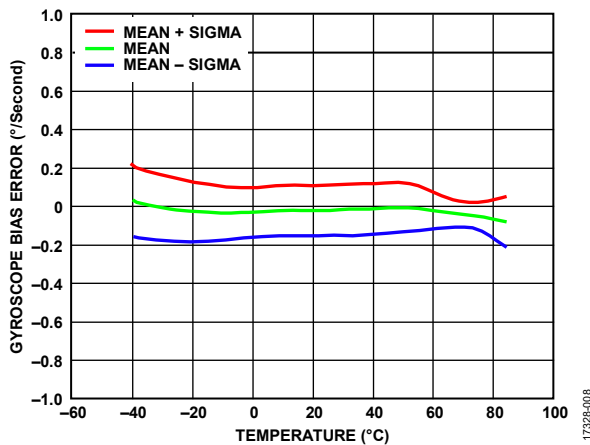
Figure 11. Gyroscope Bias Error vs. Temperature, ADIS16505-2, All Axes
