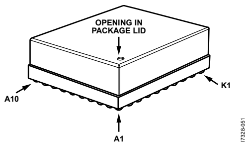
Figure 61. Pressure Relief Hole
