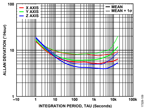
Figure 9. Gyroscope Allan Deviation, T_C = 25^\circ\text{C} , ADIS16505-3, Plot Taken After 10 Hours of Settling Time
