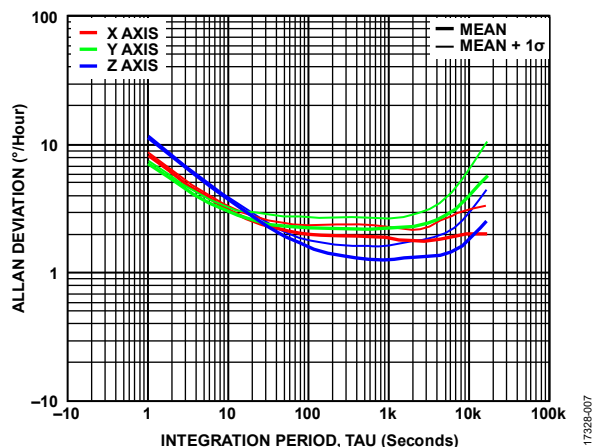
Figure 8. Gyroscope Allan Deviation, T_C = 25^\circ\text{C} , ADIS16505-2, Plot Taken After 10 Hours of Settling Time
