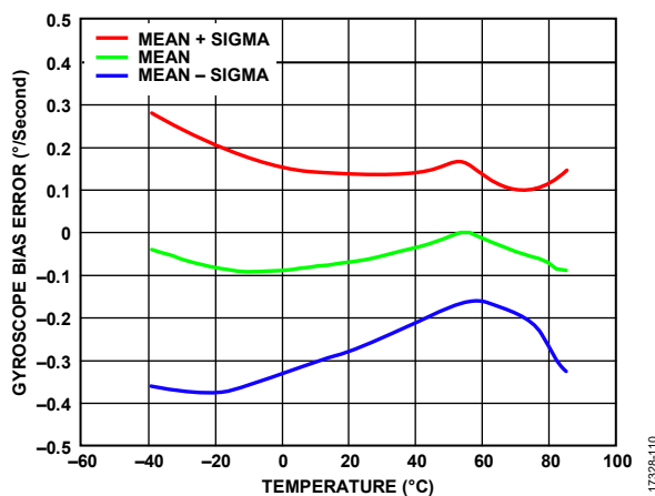
Figure 10. Gyroscope Bias Error vs. Temperature, ADIS16505-1, All Axes
