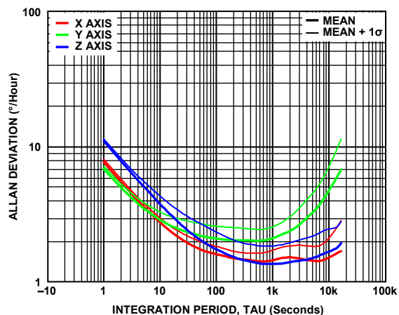
Figure 7. Gyroscope Allan Deviation, T_C = 25^\circ\text{C} , ADIS16505-1, Plot Taken After 10 Hours of Settling Time
