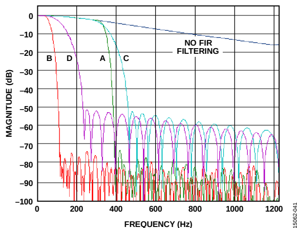
Figure 45. FIR Filter Frequency Response Curves
