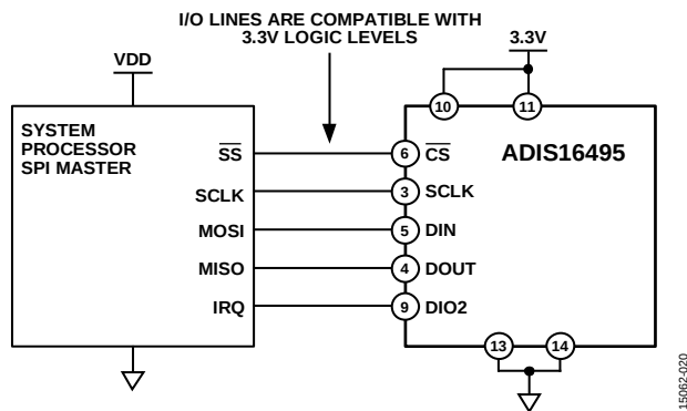
Figure 24. Electrical Connection Diagram
