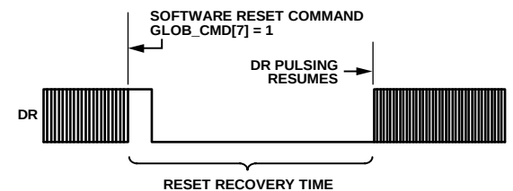
Figure 27. Data Ready Response During Reset (Register GLOB_CMD, Bit 7 = 1) Recovery
