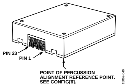
Figure 44. Point of Percussion Reference Point
