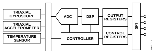
Figure 22. Basic Operation
