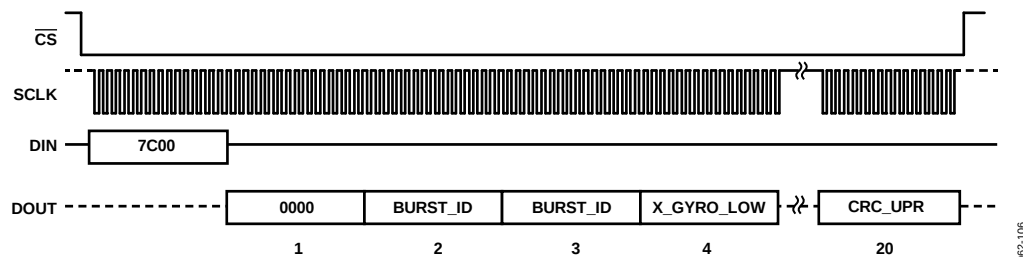
Figure 6. Burst Read Function Sequence Diagram, 20 Segments
