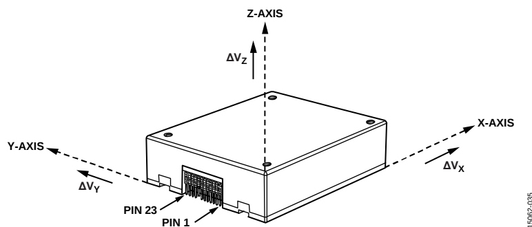
Figure 40. Delta Velocity Axis and Polarity Assignments
