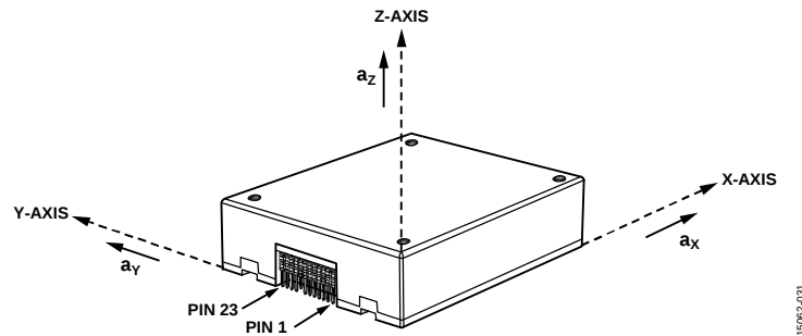
Figure 35. Accelerometer Axis and Polarity Assignments
