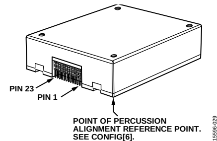
Figure 32. Point of Percussion Reference Point
