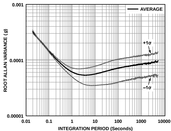
Figure 8. Accelerometer Allan Variance, T_c = 25^\circ\text{C}
