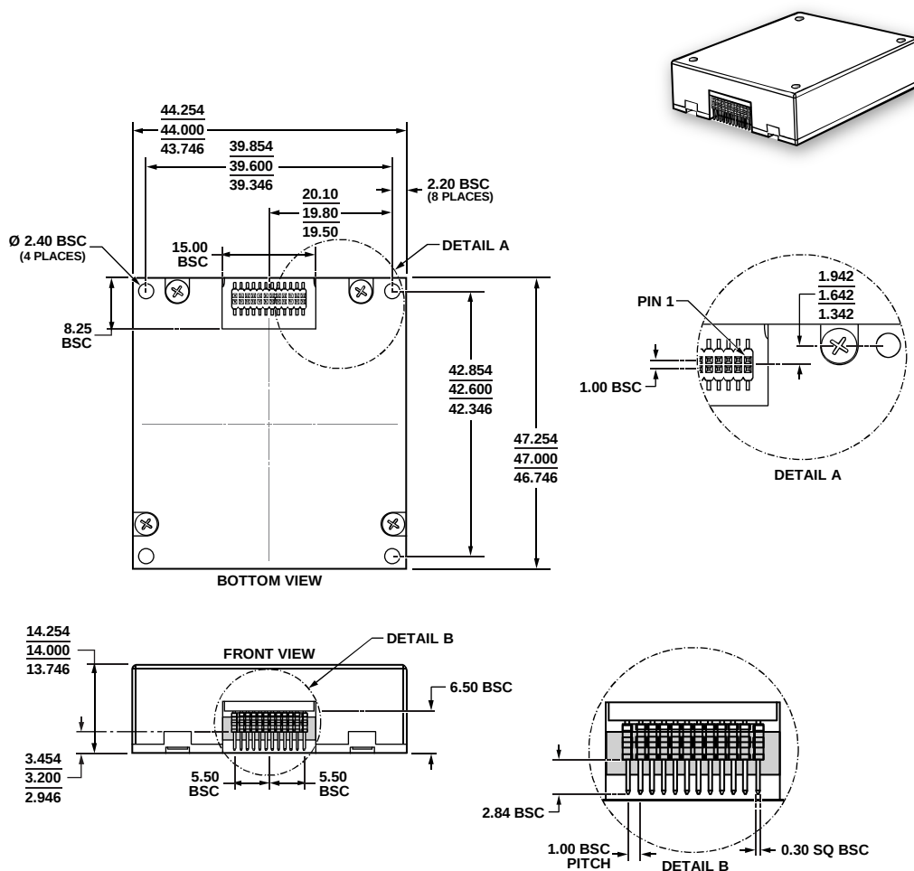
Figure 40. 24-Lead Module with Connector Interface [MODULE] (ML-24-6)
