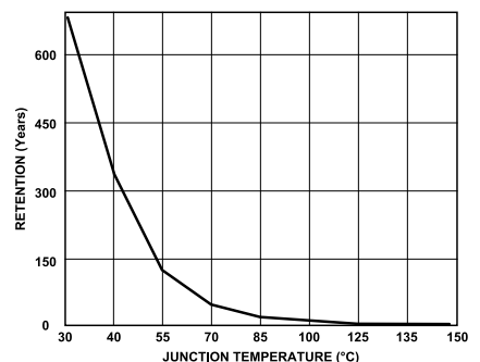
Figure 49. Flash Memory Retention
