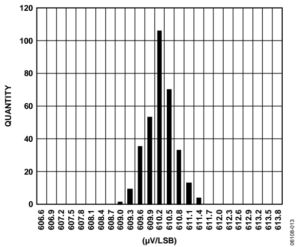
Figure 13. DAC Gain Distribution at 25°C/3.3 V
