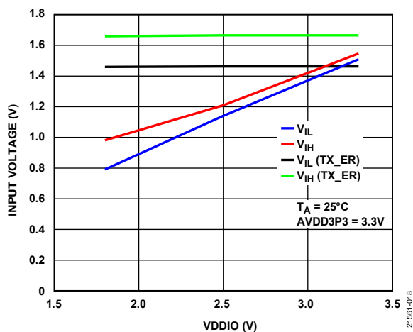
Figure 19. Digital Input Trip Levels vs. VDDIO
