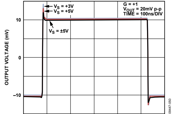
Figure 25. Small Signal Transient Response for Various Supplies, G = +1
