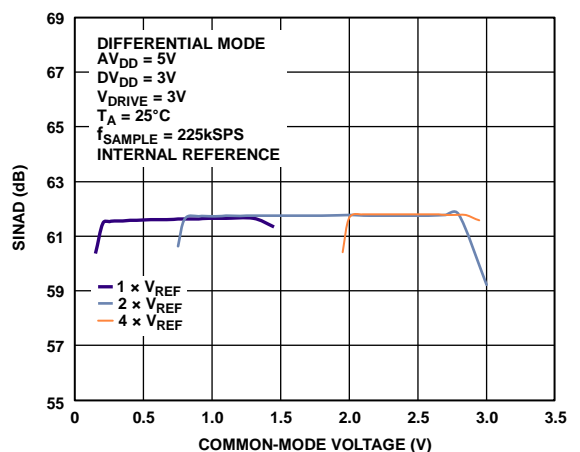
Figure 33. Common-Mode Voltage (Dependent on Input Range)
