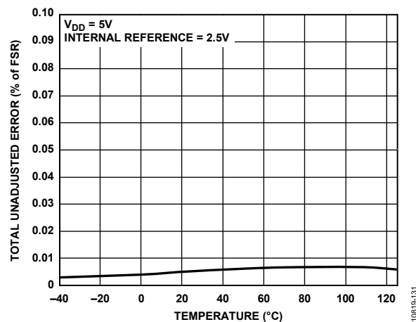
Figure 20. TUE vs. Temperature
