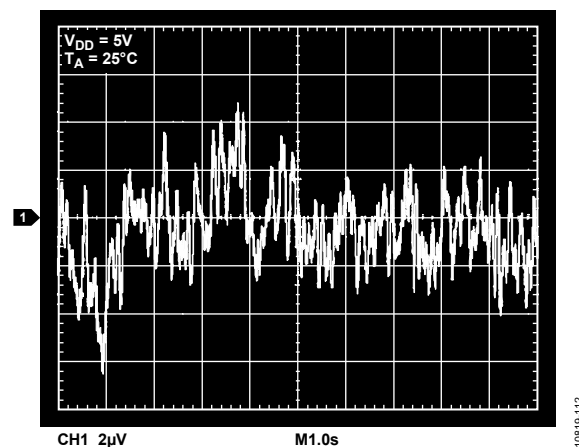
Figure 8. Internal Reference Noise, 0.1 Hz to 10 Hz
