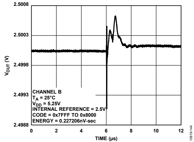
Figure 32. Digital-to-Analog Glitch Impulse
