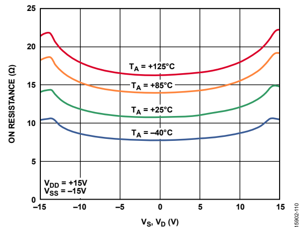
Figure 10. R_{ON} as a Function of V_S and V_D for Different Temperatures, \pm 15 V Dual Supply
