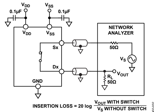
Figure 34. Bandwidth
