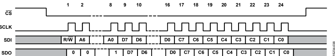
Figure 40. Timing Diagram with CRC Enabled
