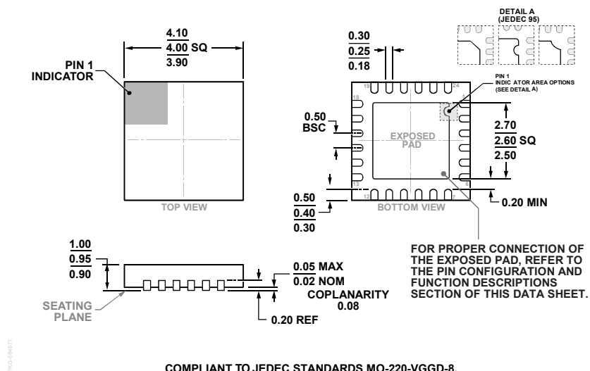
Figure 48. 24-Lead Lead Frame Chip Scale Package [LFCSP] 4 mm × 4 mm Body and 0.95 mm Package Height (CP-24-17)
