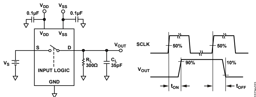
Figure 36. Switching Times
