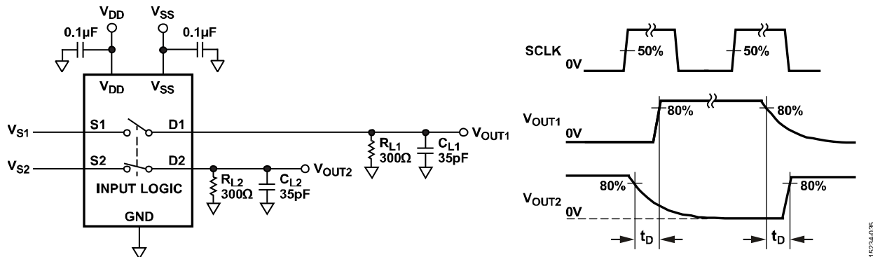
Figure 35. Break-Before-Make Time Delay, t_D
