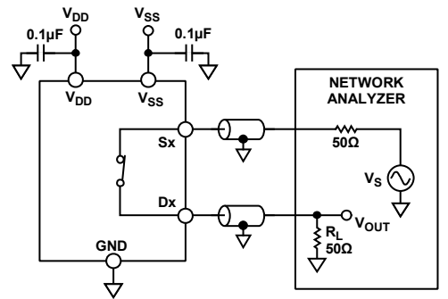
Figure 37. -3 dB Bandwidth
