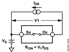
Figure 32. On Resistance
