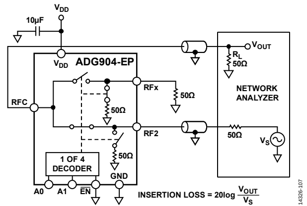
Figure 18. Insertion Loss
