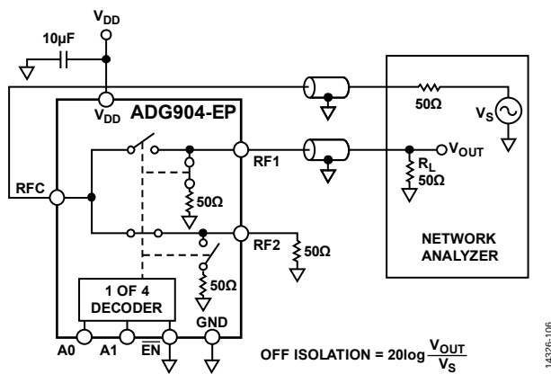
Figure 17. Off Isolation
