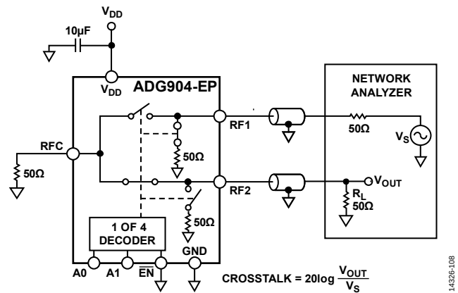
Figure 19. Crosstalk
