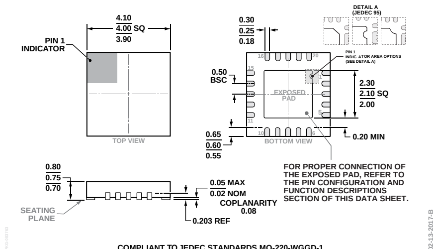
Figure 23. 20-Lead Lead Frame Chip Scale Package [LFCSP] 4 mm × 4 mm Body and 0.75 mm Package Height (CP-20-6) Dimensions shown in millimeters
