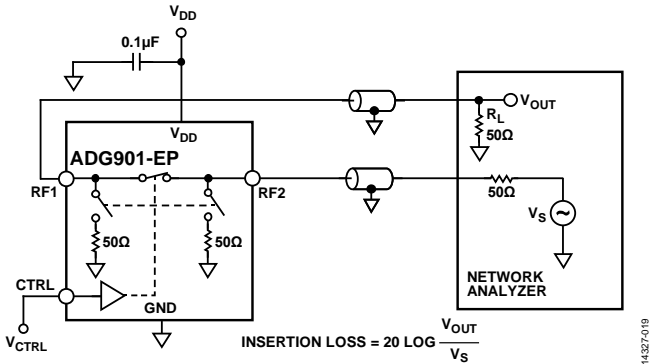
Figure 19. Insertion Loss
