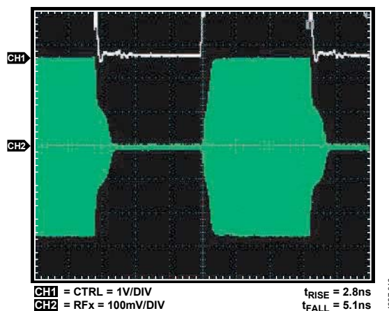
Figure 12. Switch Timing
