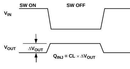
Figure 23. Charge Injection
