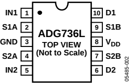
Figure 2. Pin Configuration
