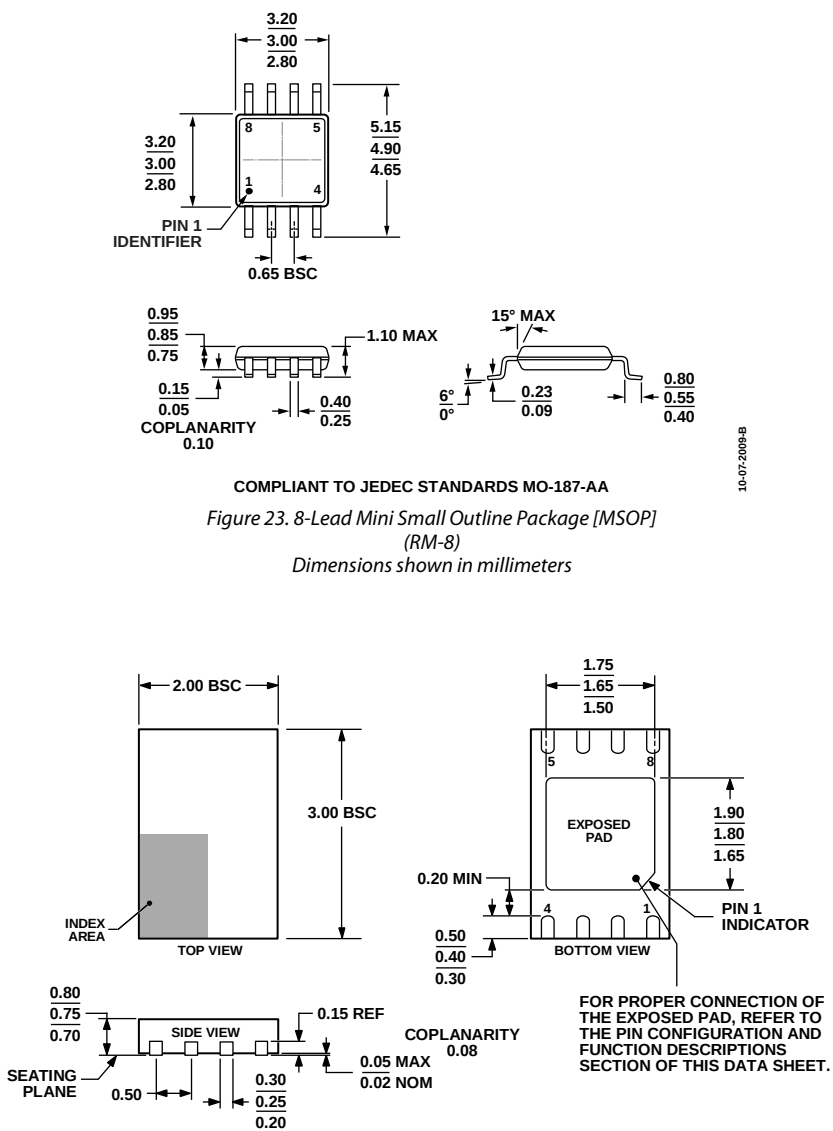
Figure 24. 8-Lead Lead Frame Chip Scale Package [LFCSP_WD] 3 mm x 2 mm Body, Very Very Thin, Dual Lead (CP-8-4) Dimensions shown in millimeters
