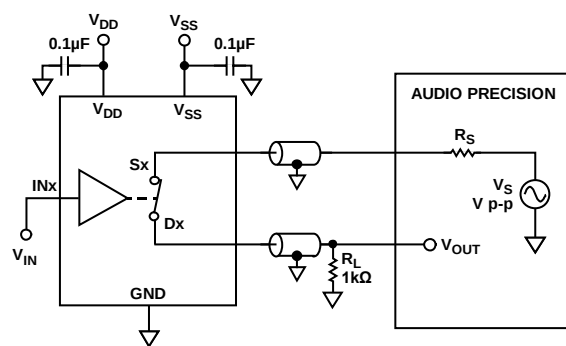
Figure 27. THD + Noise
