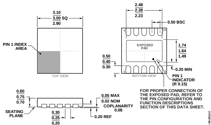
Figure 34. 10-Lead Lead Frame Chip Scale Package [LFCSP_WD] 3 mm × 3 mm Body, Very Very Thin, Dual Lead (CP-10-9)
