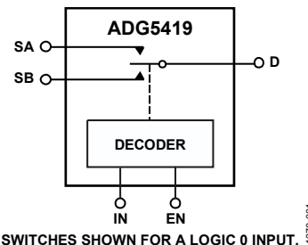
Figure 1. 8-Lead LFCSP
