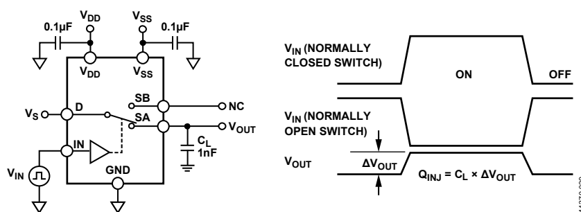
Figure 35. Charge Injection
