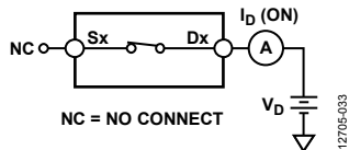
Figure 32. On Leakage
