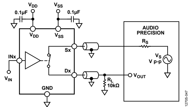
Figure 38. THD + N
