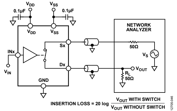
Figure 37. Bandwidth
