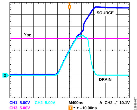
Figure 28. Drain Output Response to Positive Overvoltage
