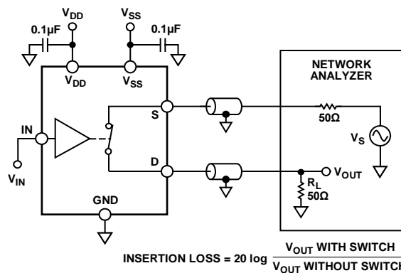
Figure 35. Bandwidth
