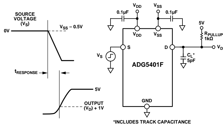
Figure 38. Negative Overvoltage Response Time, Single-Supply, t_{\text{RESPONSE}}
