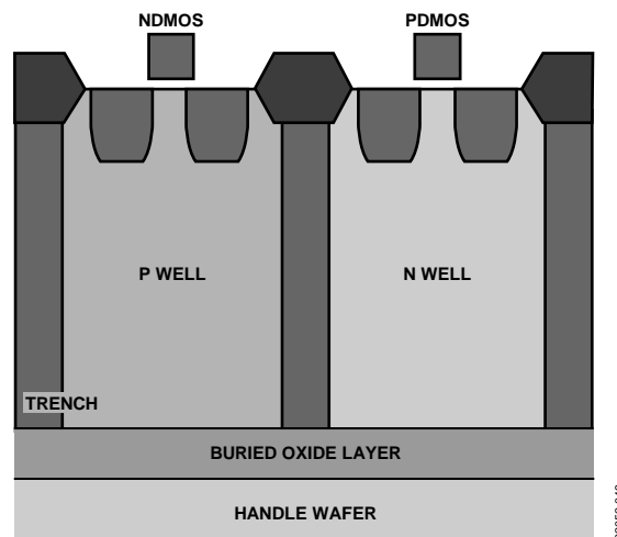
Figure 45. Trench Isolation
