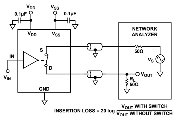
Figure 25. Bandwidth
