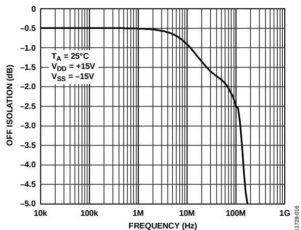
Figure 17. Bandwidth
