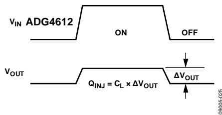
Figure 27. Charge Injection
