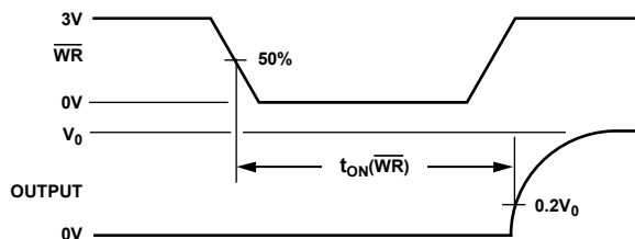
Figure 32. Write Turn-On Time, t_{ON}(\overline{WR})
