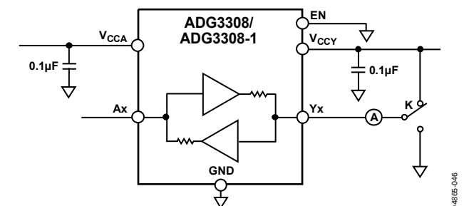
Figure 32. Three-State Leakage Current at Pin Y
