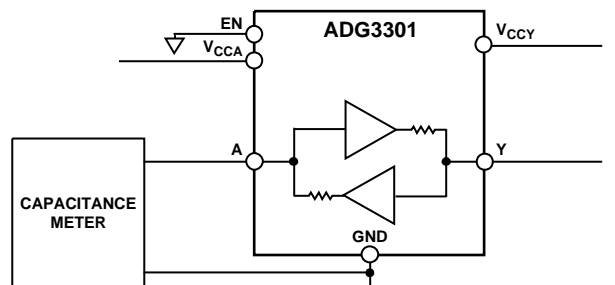
Figure 32. Capacitance at Pin A
