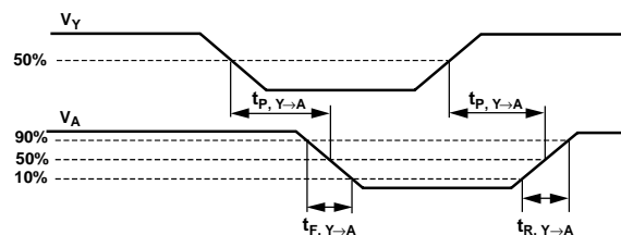
Figure 36. Switching Characteristics (Y→A Level Translation)
