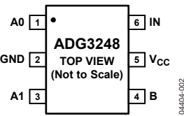
Figure 2. 6-Lead SC70
