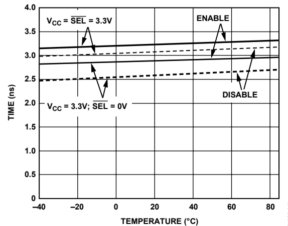
Figure 19. Enable/Disable Time vs. Temperature
