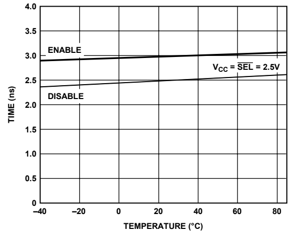
Figure 20. Enable/Disable Time vs. Temperature
