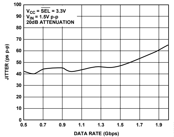
Figure 21. Jitter vs. Data Rate; PRBS 31
