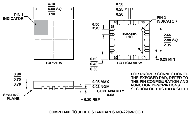
Figure 38. 20-Lead Lead Frame Chip Scale Package [LFCSP] 4 mm × 4 mm Body and 0.75 mm Package Height (CP-20-10) Dimensions shown in millimeters
