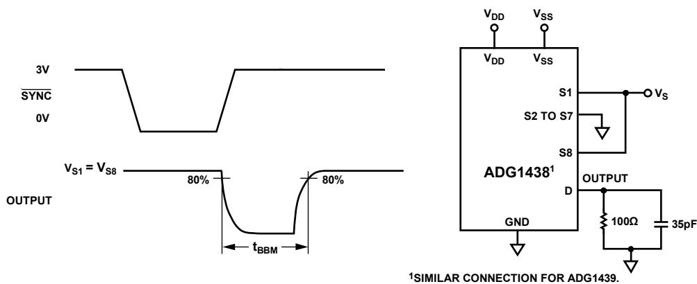
Figure 31. Break-Before-Make Delay, t_{BBM}
