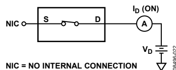
Figure 29. On Leakage
