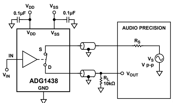
Figure 36. THD + Noise
