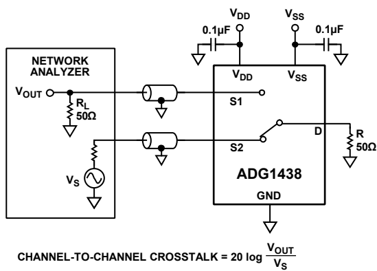
Figure 34. Channel-to-Channel Crosstalk
