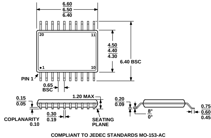
Figure 37. 20-Lead Thin Shrink Small Outline Package [TSSOP] (RU-20) Dimensions shown in millimeters
