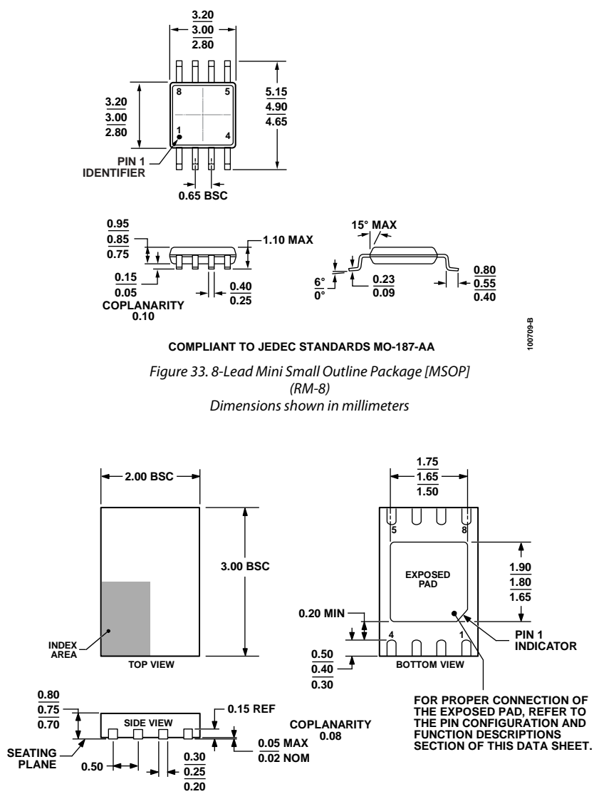
Figure 34. 8-Lead Lead Frame Chip Scale Package [LFCSP_WD] 3 mm x 2 mm Body, Very Very Thin, Dual Lead (CP-8-4) Dimensions shown in millimeters
