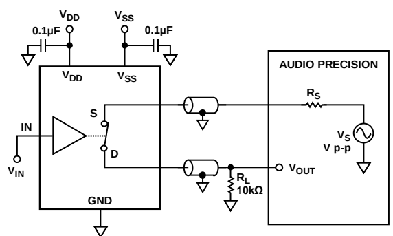
Figure 22. THD + Noise
