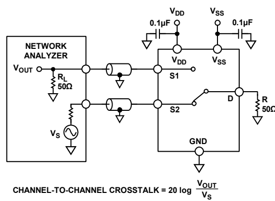
Figure 36. Channel-to-Channel Crosstalk
