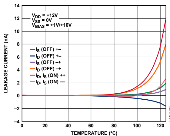
Figure 16. Leakage Current as a Function of Temperature, 12 V Single Supply
