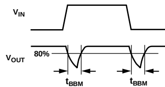
Figure 15. Break-Before-Make Delay
