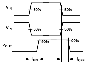
Figure 14. Switching Timing
