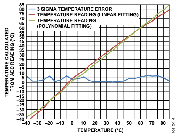
Figure 68. Temperature Sensor Performance (Average of 1000 ADC Readbacks) and 3\text{-}\Sigma Error vs. Temperature, V_{\text{DD\_BAT}} = 3.6 \text{ V}
