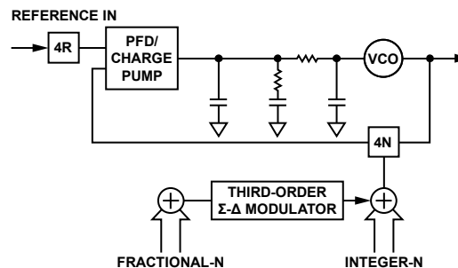
Figure 23. Fractional-N PLL
