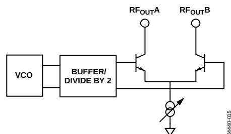
Figure 15. ADF4360-6 Output Stage
