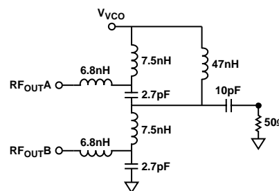
Figure 23. Balun for Combining ADF4360-6 RF Outputs
