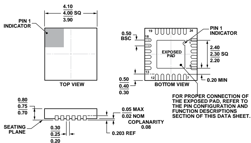
Figure 23. 24-Lead Lead Frame Chip Scale Package [LFCSP] 4 mm × 4 mm Body and 0.75 mm Package Height (CP-24-14)
