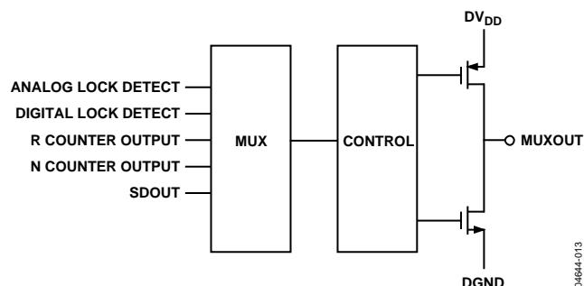
Figure 13. MUXOUT Circuit
