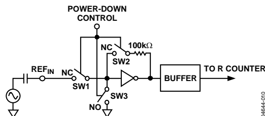
Figure 10. Reference Input Stage
