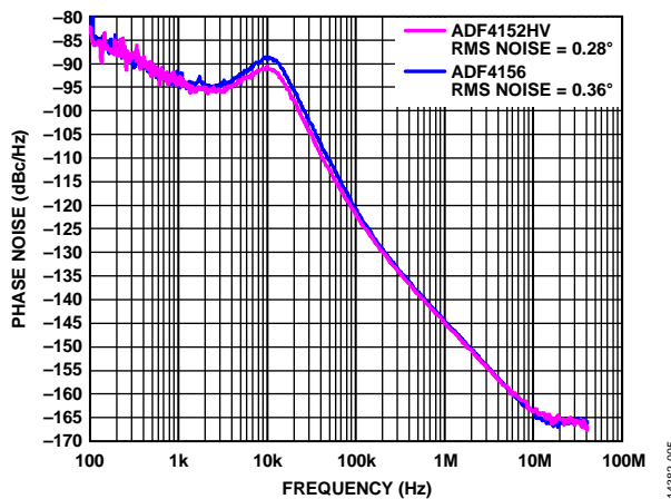
Figure 6. Active Filter Phase Noise, ADF4152HV vs. ADF4156; Active Filter Implemented Using OP27 Op Amp; PFD = 20 MHz, Loop Bandwidth = 10 kHz, I_{CP} = 300 \mu A , Carrier Frequency = 1.7 GHz, V_P = 28 V
