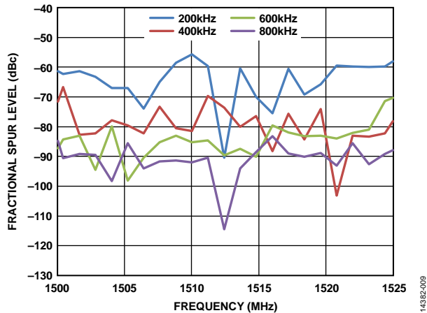
Figure 10. Fractional Spur Levels vs. Frequency, Low Noise Mode; Measured at VCO Output, PFD = 25 MHz, MOD = 125
