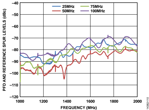
Figure 11. PFD and Reference Spur Levels vs. Frequency, Measured at VCO Output, REF_{IN} = 100 MHz, PFD = 25 MHz
