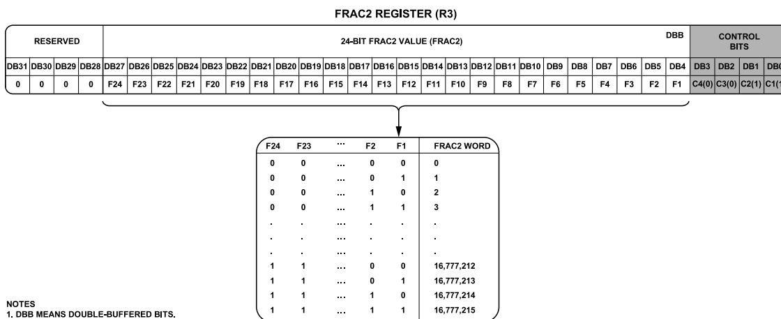
Figure 26. Register 3 (R3) Map
