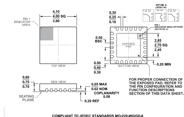
Figure 38. 24-Lead Lead Frame Chip Scale Package [LFCSP] 4 mm × 4 mm Body and 0.75 mm Package Height (CP-24-8) Dimensions shown in millimeters
