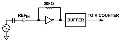
Figure 14. Reference Input Stage
