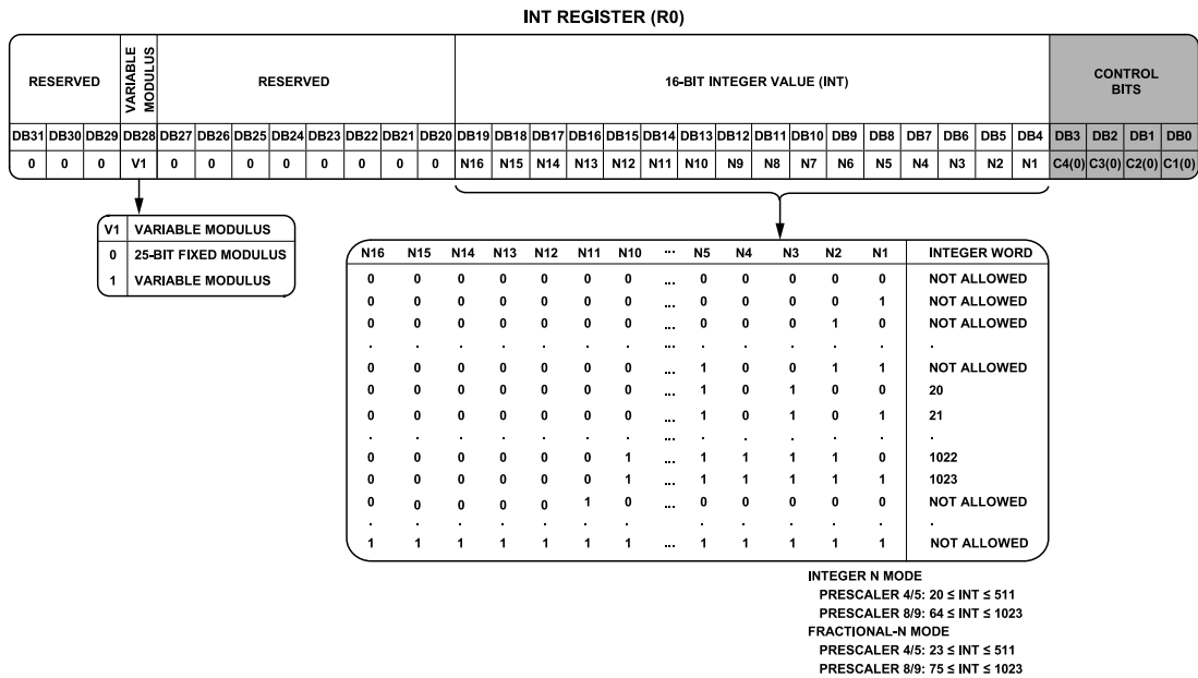
Figure 23. Register 0 (R0) Map
