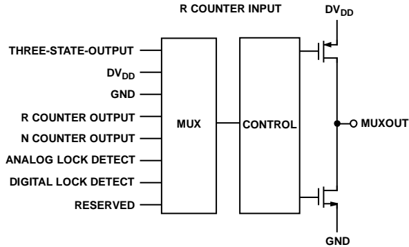
Figure 17. MUXOUT Schematic
