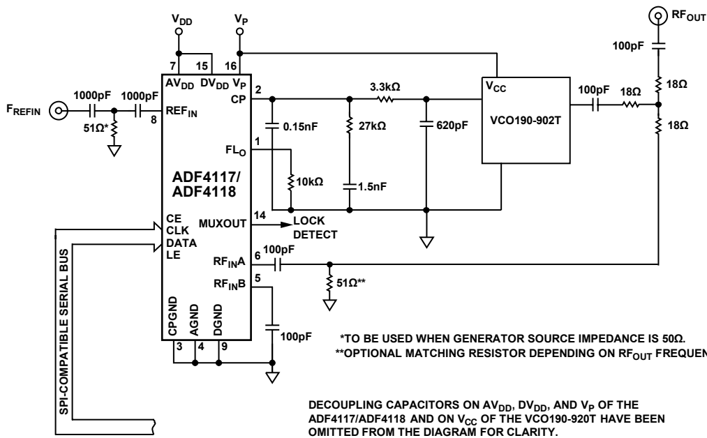
Figure 35. Local Oscillator for GSM Base Station
