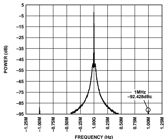
Figure 8. Reference Spurs (RF = 1000 MHz, PFD = 1 MHz)
