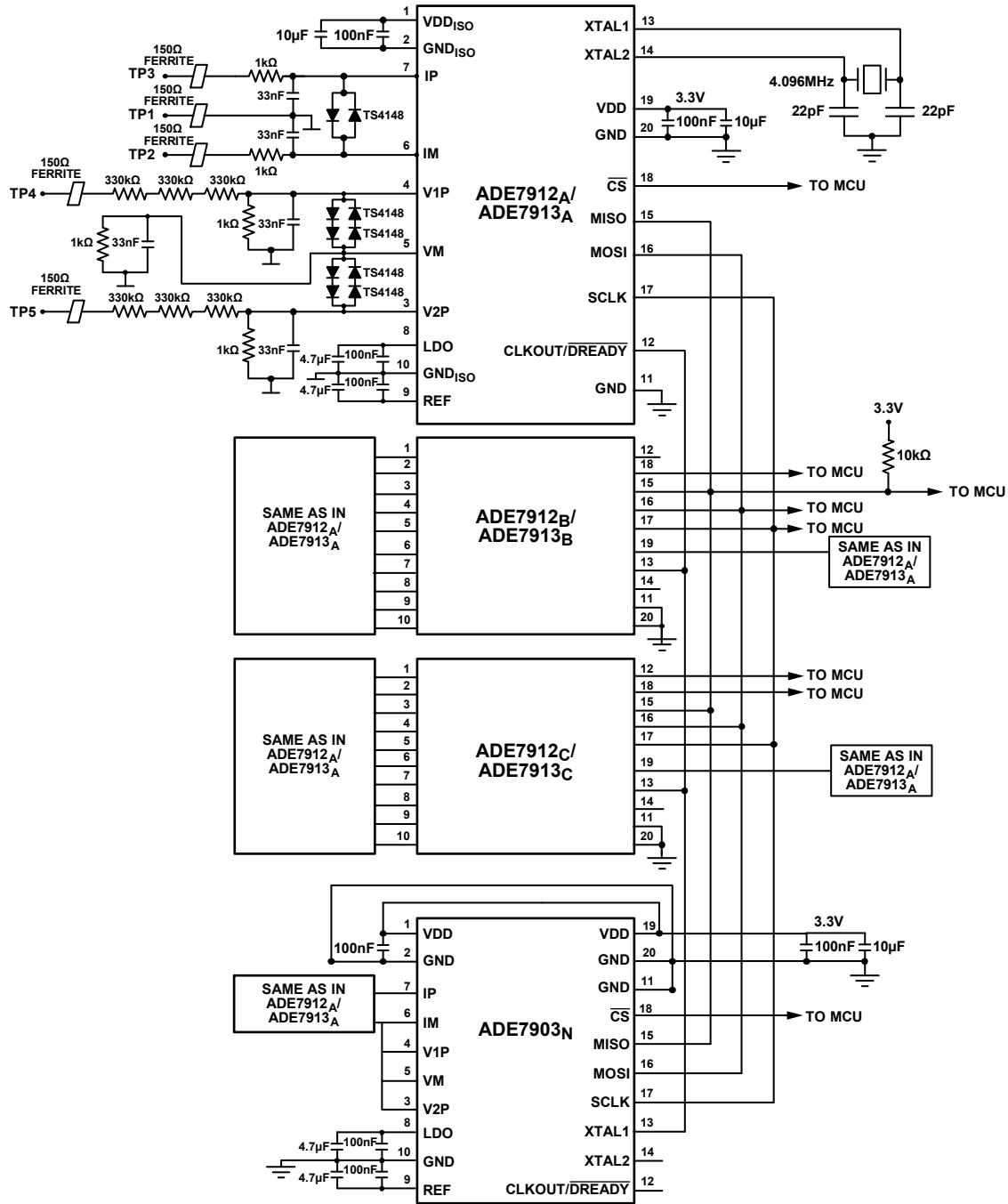
Figure 18. Test Circuit
