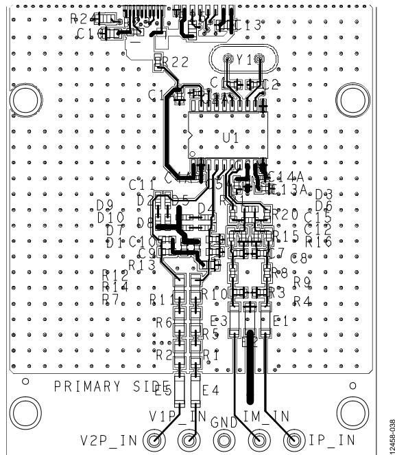
Figure 38. 2-Layer Circuit Board, Top Layer
