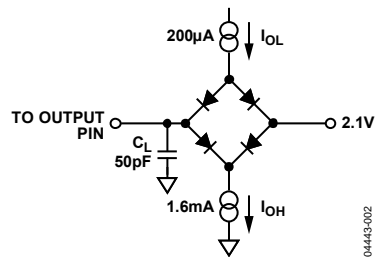
Figure 2. Load Circuit for Timing Specifications
