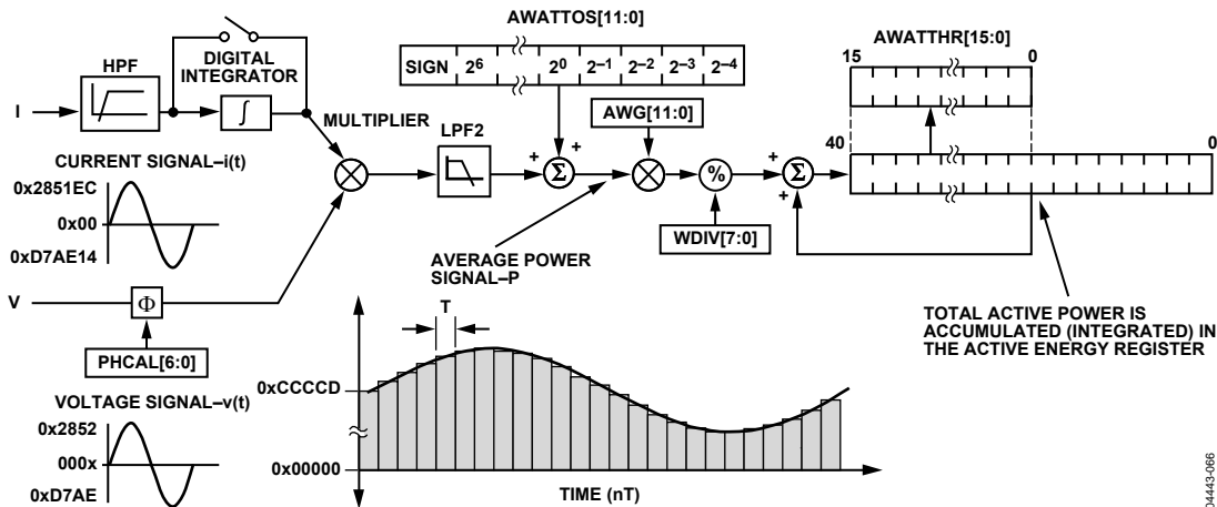
Figure 67. ADE7758 Active Energy Accumulation
