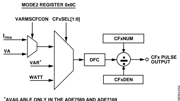
Figure 79. Energy to Frequency Conversion
