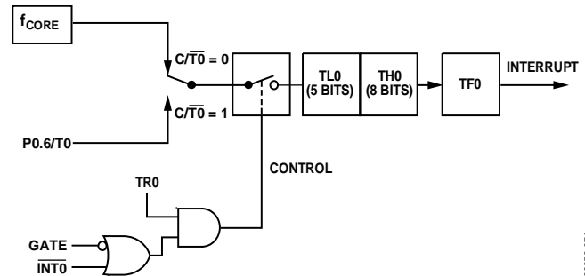
Figure 97. Timer/Counter 0, Mode 0
