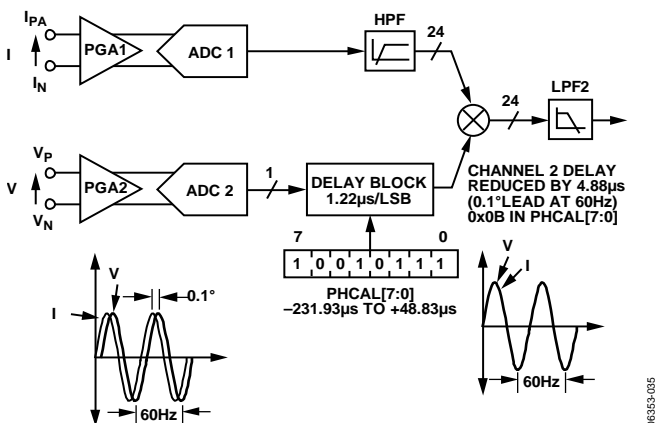
Figure 59. Phase Calibration
