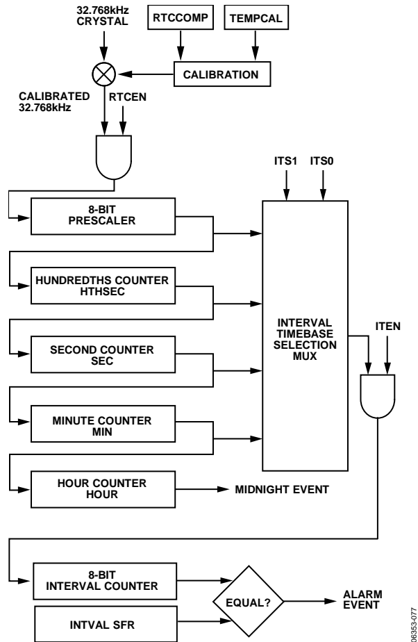
Figure 103. RTC Implementation
