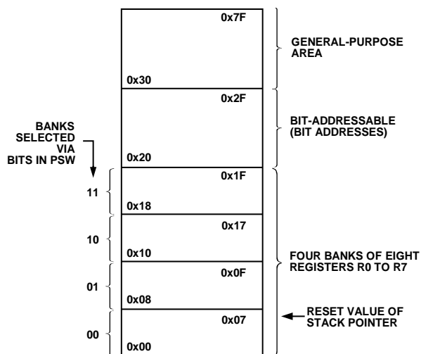
Figure 83. Lower 128 Bytes of Internal Data Memory
