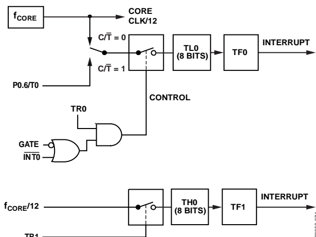
Figure 100. Timer/Counter 0, Mode 3
