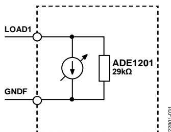
Figure 30. Programmable Load Current Block Diagram
