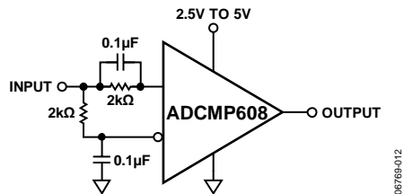
Figure 12. Self-Biased, 50% Slicer
