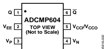
Figure 3. ADCMP604 Pin Configuration
